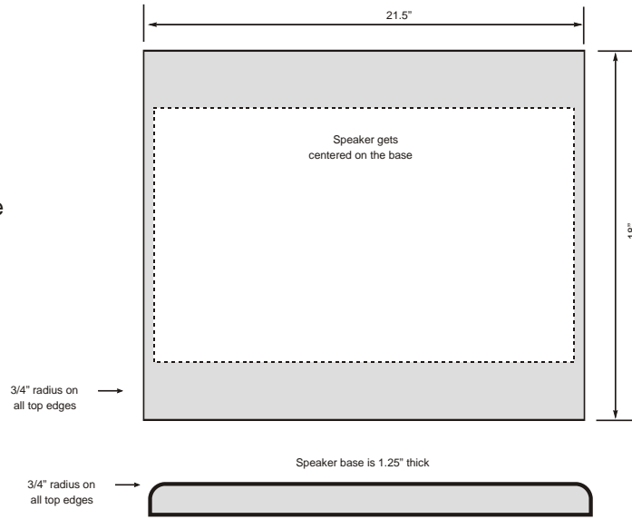
Speaker base
